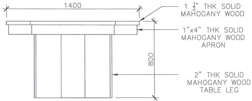
TYPICAL FRONT AND REAR VIEW
